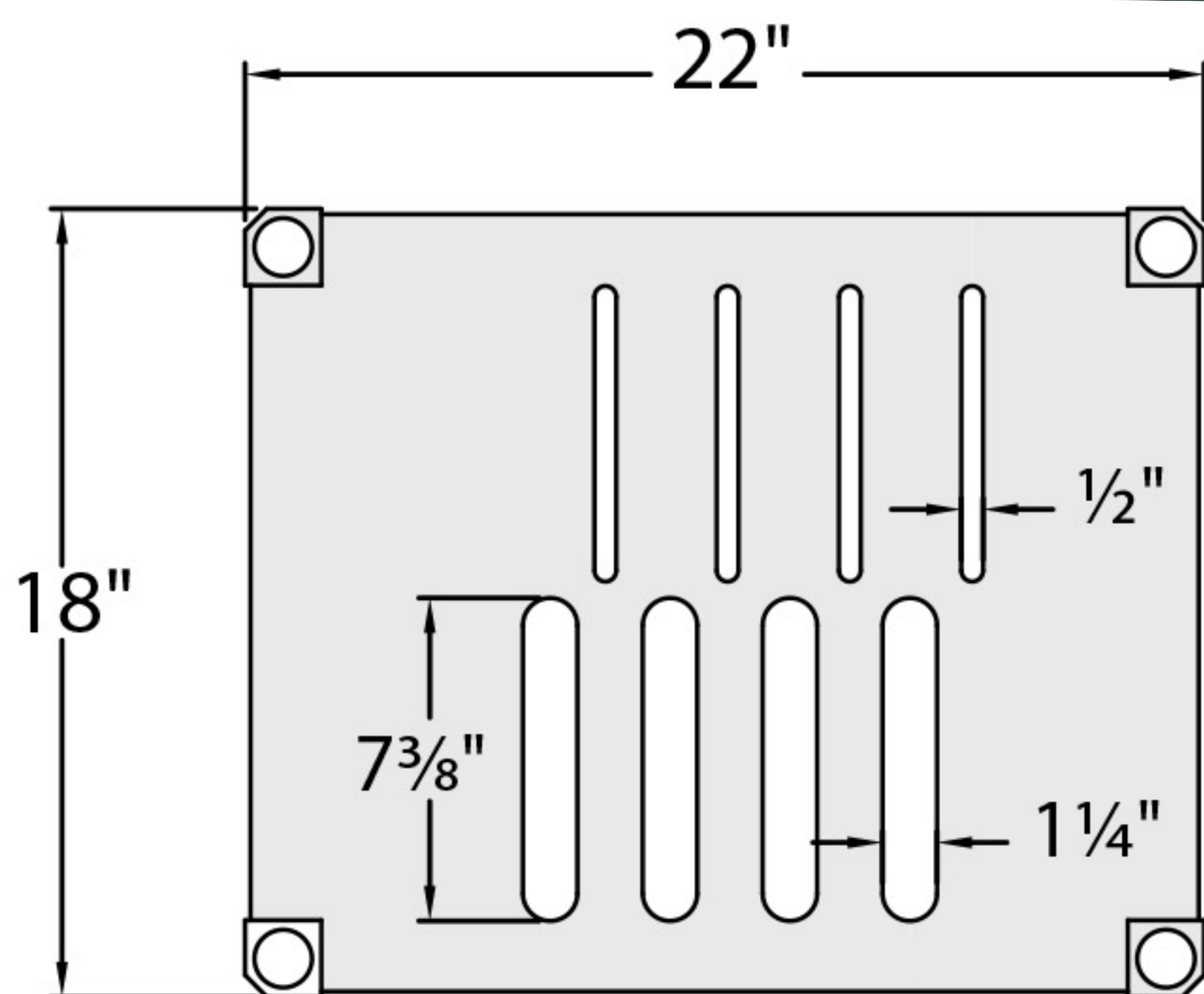
Lower Shelf Layout Holds (10) Cutting Discs
